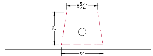
SIDE POCKET ELEVATION
