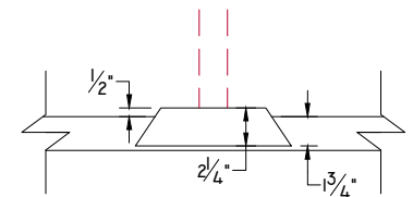
SIDE POCKET PLAN VIEW
