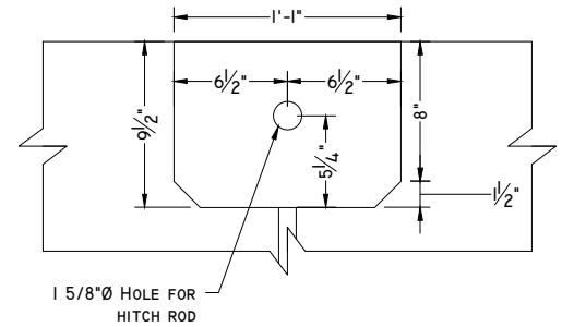
HITCH ROD POCKET ELEVATION
