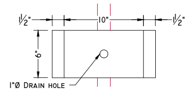
HITCH ROD POCKET PLAN VIEW
