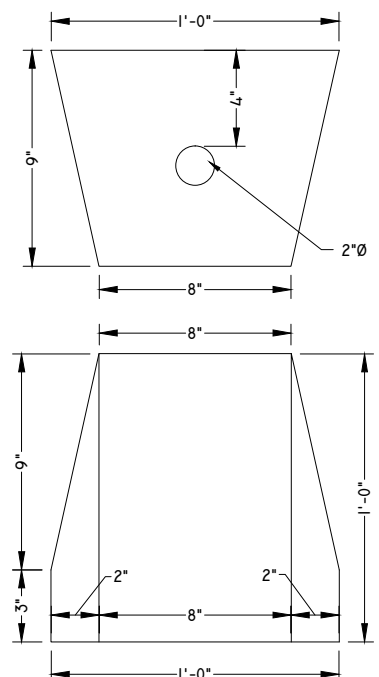
SIDE POCKET DETAIL
