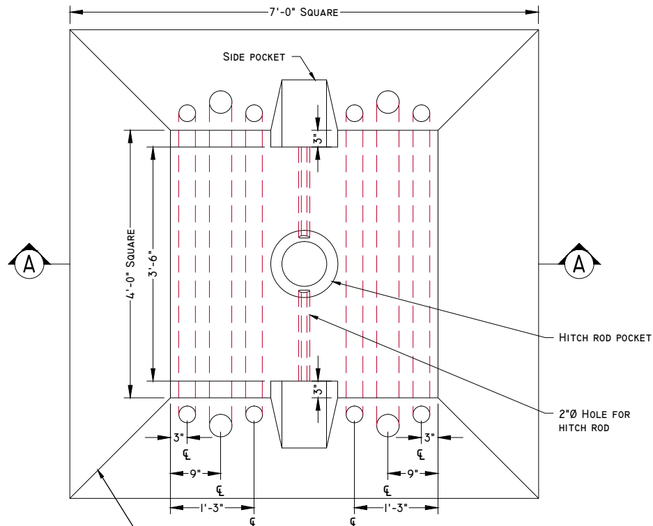
PLAN VIEW
